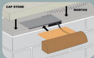
CAST Set-in-Stone® Wall Light Mounting System (for CEWL5 Series)
