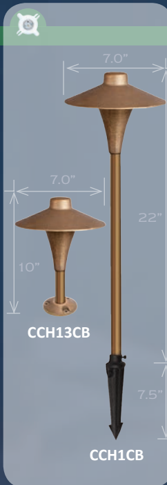
Small China Hat (CCH1CB, CCH13CB)
